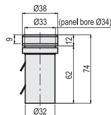
Battery case
