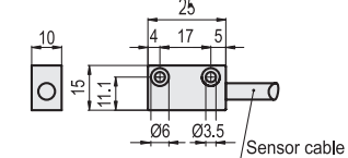
Magnetic sensor
